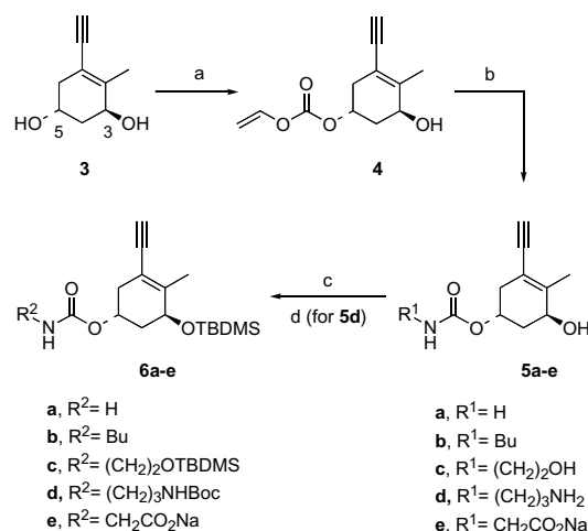
Scheme 1. Reagents and conditions: (a) CAL-B, acetone O -[(vinyl-oxo)carbonyl]oxime, toluene, 30 °C, 4 h (quantitative); (b) \text{R}^1\text{NH}_2 , THF (DMF for 5e ), 60 °C [18 h (quantitative) for 5a , 22 h (91%) for 5b , 48 h (80%) for 5c , 48 h (76%) for 5d , 48 h (87%) for 5e ]; (c) TBDMSCl, imidazol, DMAP, \text{CH}_2\text{Cl}_2 , rt, 12 h (91% for 6a , 97% for 6b , 86% for 6c , 88% for 6e ); (d) \text{Boc}_2\text{O} , \text{CHCl}_3 , \text{NaHCO}_3 (aq), rt, 3 h (67% for 6d , steps c and d).
