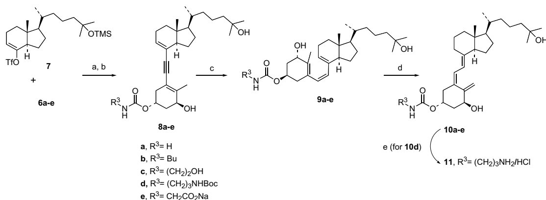
Scheme 2. Reagents and conditions: (a) Pd(PPh_3)_4(OAc)_2 , CuI, Et_2NH , DMF, rt, 1 h; (b) Bu_4NF , THF, rt, 12 h (90% for 8a , 71% for 8b , 90% for 8c , 96% for 8d , 61% for 8e , two steps); (c) H_2 , Lindlar cat., quinoline, MeOH, rt, 1 h; (d) acetone, 80 °C, 4 h (65 °C, 3 h for 9e ) (62% for 10a , 54% for 10b , 71% for 10c , 54% for 10d , 62% for 10e , two steps); (e) HCl(g) , EtOH, rt, 30 min (69%).
