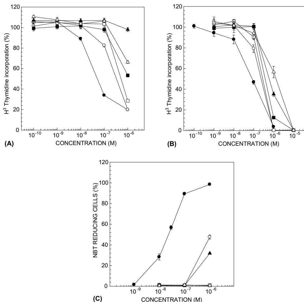
Figure 2. Prodifferentiating and antiproliferating effects of carbamate analogues on: (A) MCF-7; (B) keratinocytes; and (C) HL 60 cells. 1 \alpha ,25-(OH) 2 -D 3 (●); 10a (○); 10b (■); 10c (□); 10e (▲); 11 (△).
